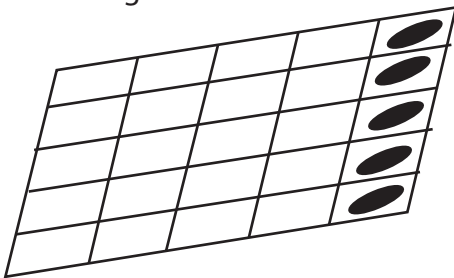
Homogeneous strain
