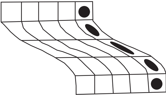
Simple Shear
