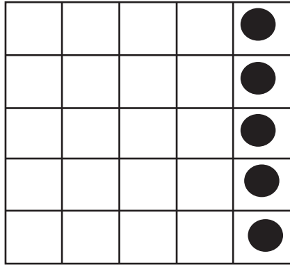
Original shape
