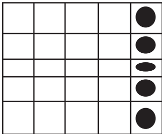
Volume change
