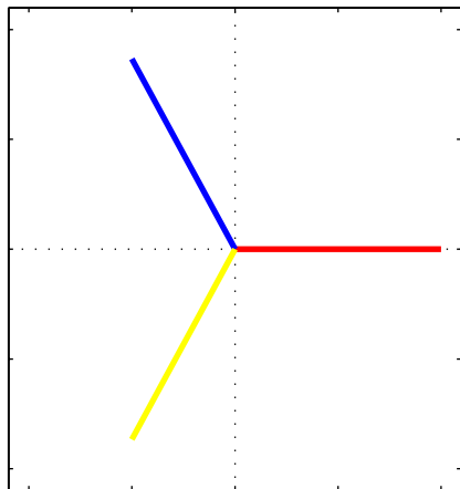
Positive Sequence Vectors
