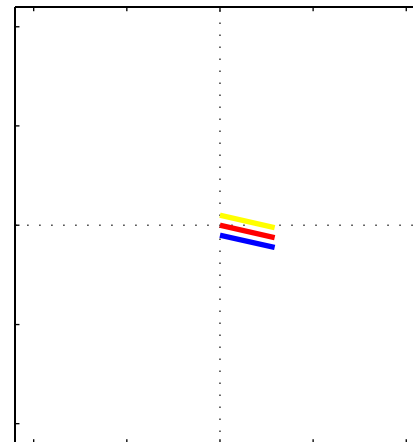
Zero Sequence Vectors
