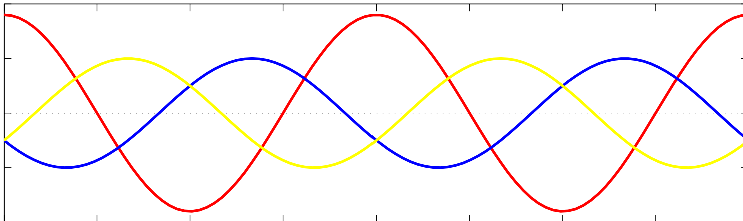
Three Unbalanced Phases
