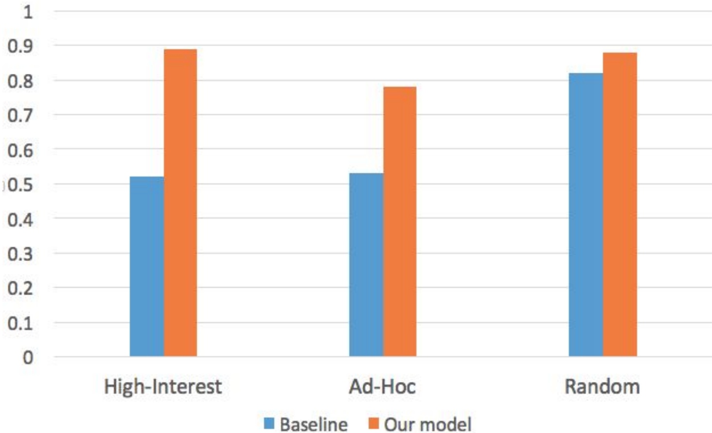
Classification accuracies across datasets, averaged across languages
