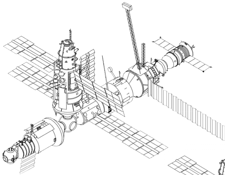
Kristall repositions up May 26, 95 Note one Kristall array retracted (60%) with the second moved to the port side of Kvant during EVAs that same month.
