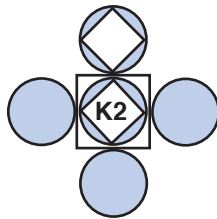
Kvant-2 (dock to -X) Dec. 6, 89
