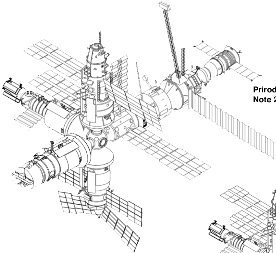
Priroda repositions to port side port Apr. 27, 96
