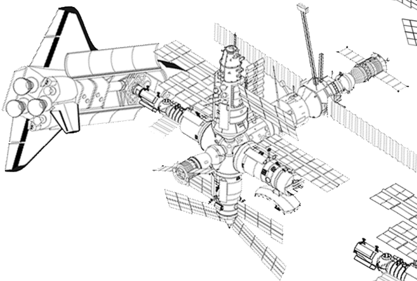
STS-79 docks to Docking Module Sep. 19, 96 Note a new Kvant array stored on the DM added to the starboard side of Kvant during EVAs In May, 1996. Also Strombus Mast replaces Rapana and Priroda Travers Parabolic Antenna unfurled. Both during an EVA on Jun. 13, 96
