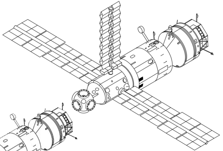
Mir mated with Kvant Apr. 9, 1987 Note third central array added in EVAs during Jun., 1987
