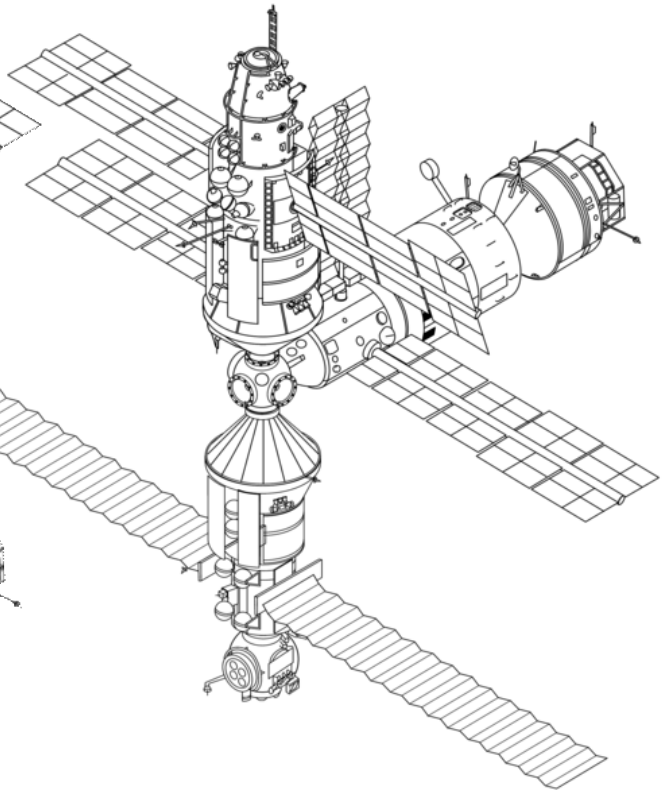
Kristall repositions to lower port Jun. 11, 1990
