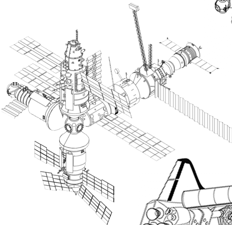
Kristall repositions to starboard port Jul. 17, 95 Note Spektr array unfurled during EVA on Jul. 14, 95
