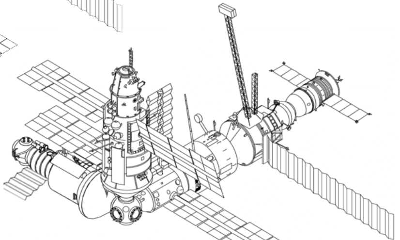
Kristall repositions to the starboard side May 29, 95
